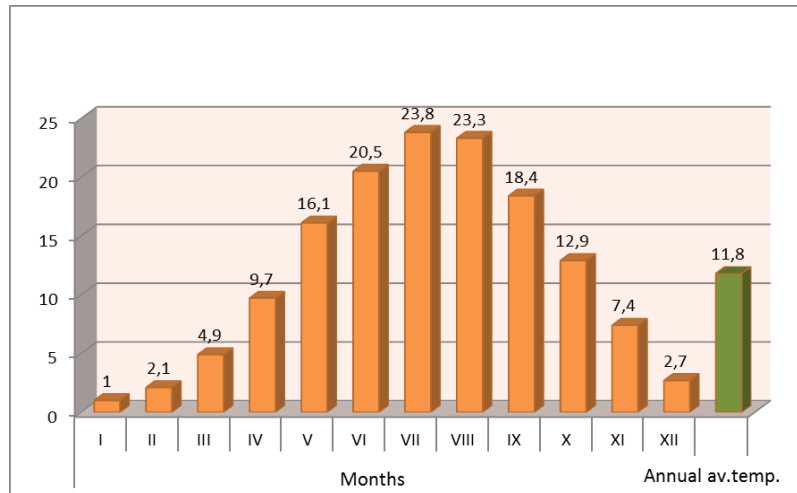
Figure 1. Average monthly and annual air temperature (°C) according to the data by Sujinka hydrometeorology station
