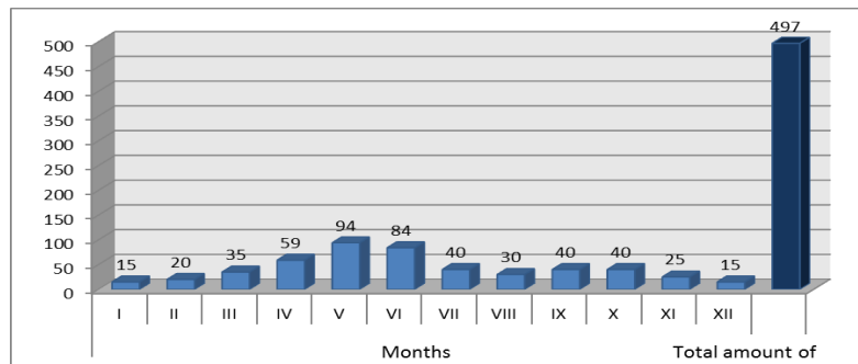
Figure 2. Average rates of monthly and annual precipitations (mm) according to the data by Sujinka hydrometeorology station
