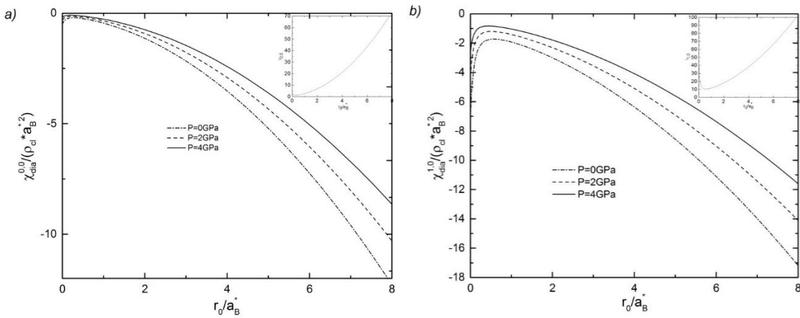
Figure 1. Dependencies of diamagnetic susceptibility \chi_{dia} on parameter r_0 for different values of hydrostatic pressure for a) 1s and b) 2s states
