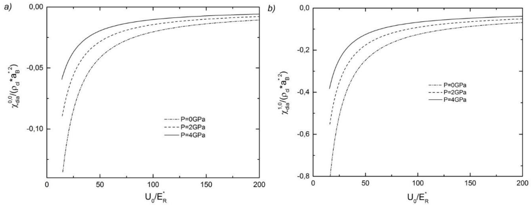
Figure 2. Dependencies of diamagnetic susceptibility \chi_{dia} on parameter U_0 for different values of hydrostatic pressure for a) 1s and b) 2s states.
